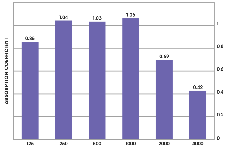
Auralex 2" PVC Wrapped ProBanner Absorption Coefficient
